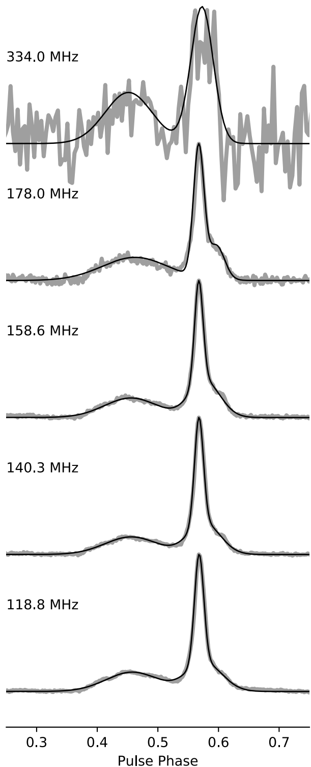
Figure 10. The integrated pulse profiles of PSR J1658+3630 at several different sub-bands obtained with the LOFAR core and at 334 MHz obtained with the Lovell Telescope. The profiles (grey) are overlaid with the models (black) that describe the profiles at different observing frequencies in order to study profile evolution.
