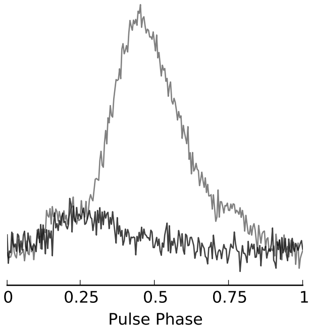
Figure 4. The integrated pulse profile of PSR J0421+3255 (grey) created by summing all available observations, except the two that show a timing offset (see Figure 1). Overlaid in black is the integrated pulse profile derived from just the two observations showing a timing offset. The difference in profile shapes suggests that there is mode changing, where the pulsar emission sometimes occurs preferentially at the leading edge of the regular emission. The integrated pulse profiles are normalized via the off-pulse standard deviation between phases 0.9 and 1.
