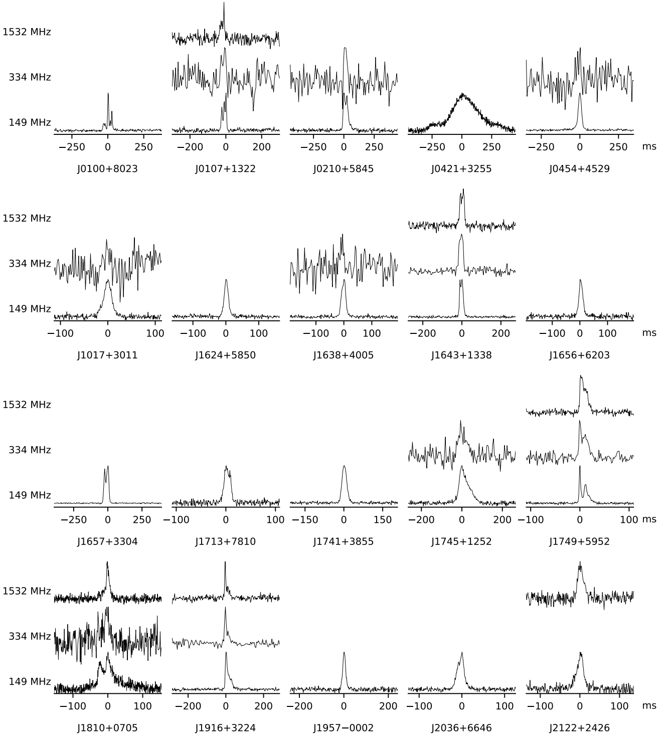
Figure 3. The pulse profiles at 149, 334 and 1532 MHz for the 20 pulsars shown in Table 3. For each profile, 50 per cent of the pulse phase is shown, except for PSRs J0421+3255 and J1810+0705, where the full pulse phase is shown. The profiles at 149 and 1532 MHz have 512 profile bins across the pulse phase, while those at 334 MHz have 256 profile bins across the pulse phase. The scales provide a reference to the width of the profiles in milliseconds.
