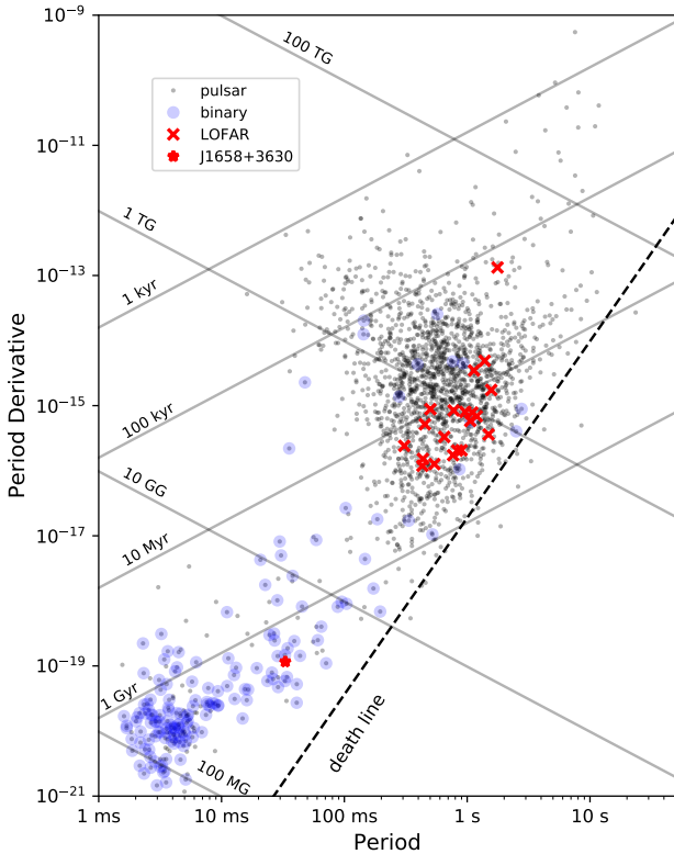
Figure 2. The P - \dot{P} -diagram of pulsars, overlaid with the 21 LOTAAS discoveries discussed here. The LOTAAS discoveries are indicated with a red cross and PSR J1658+3630 indicated with a red star. The death line plotted here is the one modelled by Equation 9 of Chen & Ruderman (1993) . Lines of constant characteristic ages and inferred surface magnetic field strengths are indicated in the plot.
