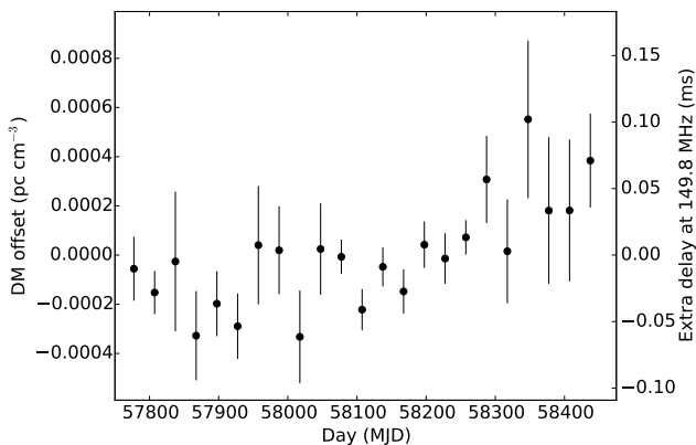
Figure 9. The modelled DM variation of PSR J1658+3630 over the observing span.
