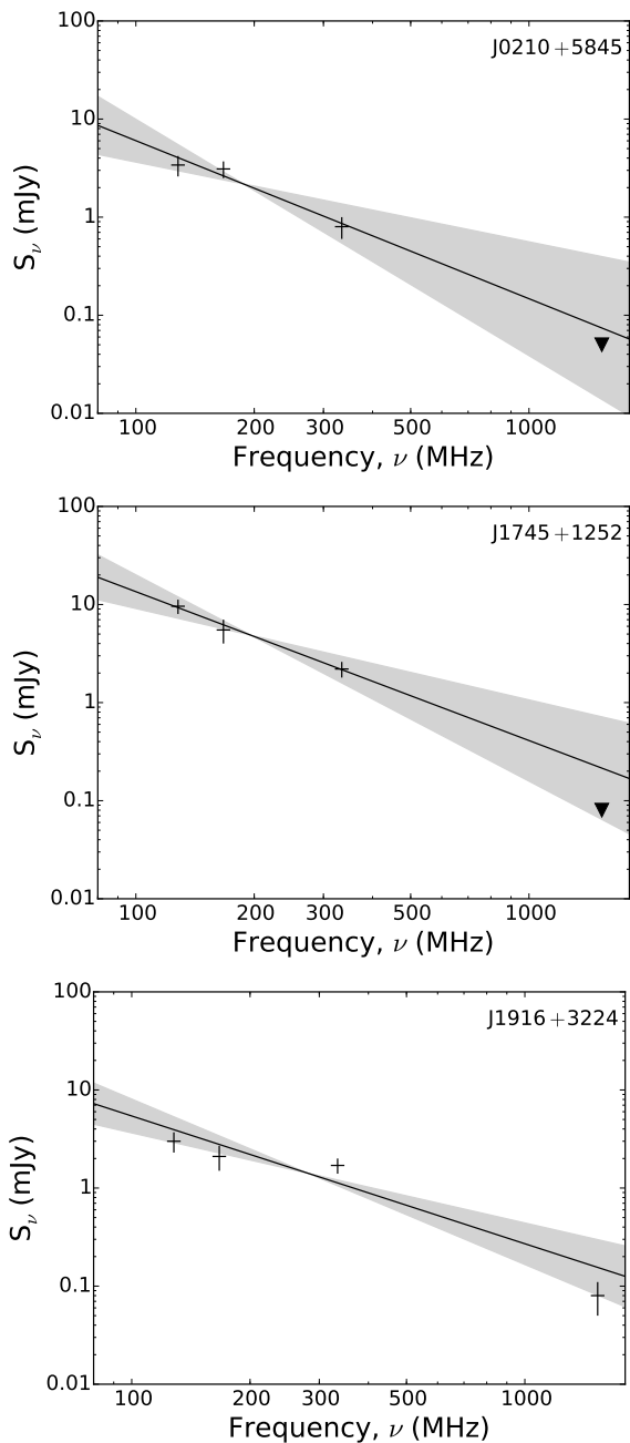
Figure 5. The spectra of PSRs J0210+5845 ( top ), J1745+1252 ( centre ) and J1916+3224 ( bottom ), fitted with a simple power law. The fitted spectral indices are shown as black lines, with a 1\sigma uncertainty region shaded in grey. The triangles denote the upper limits on flux densities from the non-detections at the relevant observing frequencies, assuming a minimum S/N detection threshold of 10. The fitted spectral indices and uncertainties can be found in Table 7.
