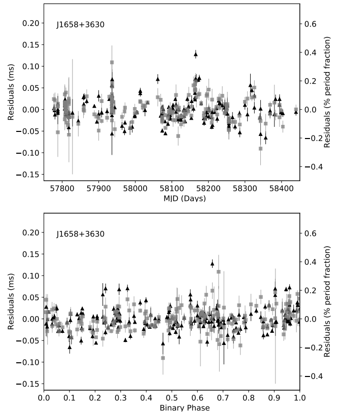
Figure 8. The timing residuals of PSR J1658+3630 over time ( top ) and in terms of the binary orbital phase of the pulsar ( bottom ). The different symbols represents the different observing frequencies, with the black triangles representing the lower part of the LOFAR and GLOW bands (central frequencies of 128 MHz and 140 MHz, respectively) and grey squares for the upper part of the LOFAR and GLOW bands (central frequencies of 167 MHz and 171 MHz, respectively).
