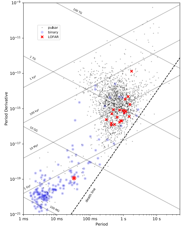
Figure 2. The P-\dot{P} -diagram of pulsars, overlaid with the 21 LOTAAS discoveries discussed here. The LOTAAS discoveries are indicated with a red cross, with PSR J1658+3630 indicated with a red cross with a circle. The death line plotted here is the one modelled by Equation 9 of Chen & Ruderman (1993).
