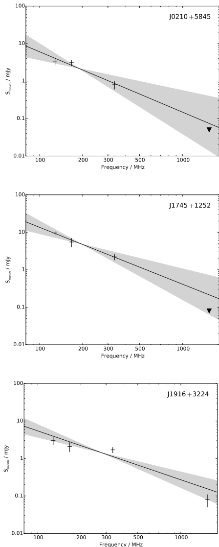
Figure 5. The spectra of PSRs J0210+5845 ( top ), J1745+1252 ( centre ) and J1916+3224 ( bottom. ), fitted with a simple power law. The fitted spectral indices are shown as black lines, with a 1\sigma uncertainty region shaded in grey. The triangles denote the upper limit in flux densities of the non-detections at the relevant observing frequencies. The fitted spectral indices and uncertainties of these pulsars can be found in Table 7.
