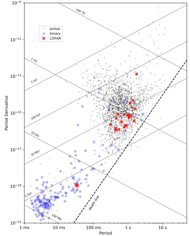
Figure 2. The P - \dot{P} -diagram of pulsars, overlaid with the 21 LOTAAS discoveries discussed here. The LOTAAS discoveries are indicated with a red cross, with PSR J1658+3630 indicated with a red cross with a circle. The death line plotted here is the one modelled by Equation 9 of Chen & Ruderman (1993) .
