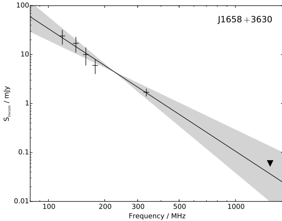
Figure 11. The spectrum of PSR J1658+3630, modelled with a single power law. The triangle is the upper limit in flux density at 1532 MHz estimated from a 1-hour non-detection with the Lovell telescope. The black line is the best-fit spectral index of -2.5 and the grey shaded region is the 1\sigma uncertainty in the fitted spectral index.
